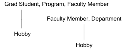
Figure 2: Sample Scheme-Tree Forest for the Diagram in Figure 1
