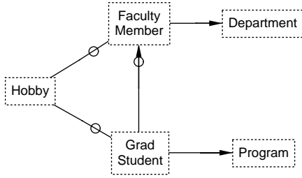
Figure 1: Simple Faculty-Student-Hobbies Diagram
